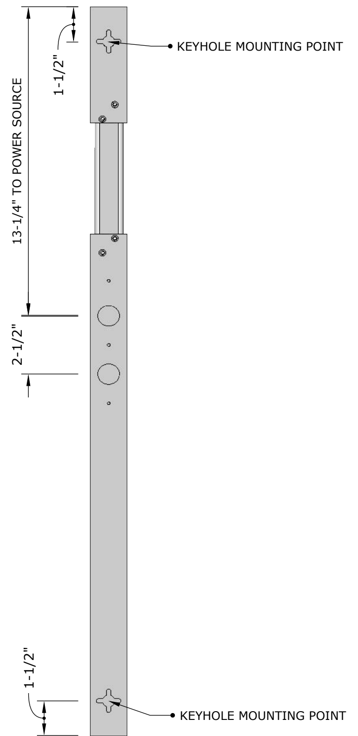
MOUNTING DETAILS
